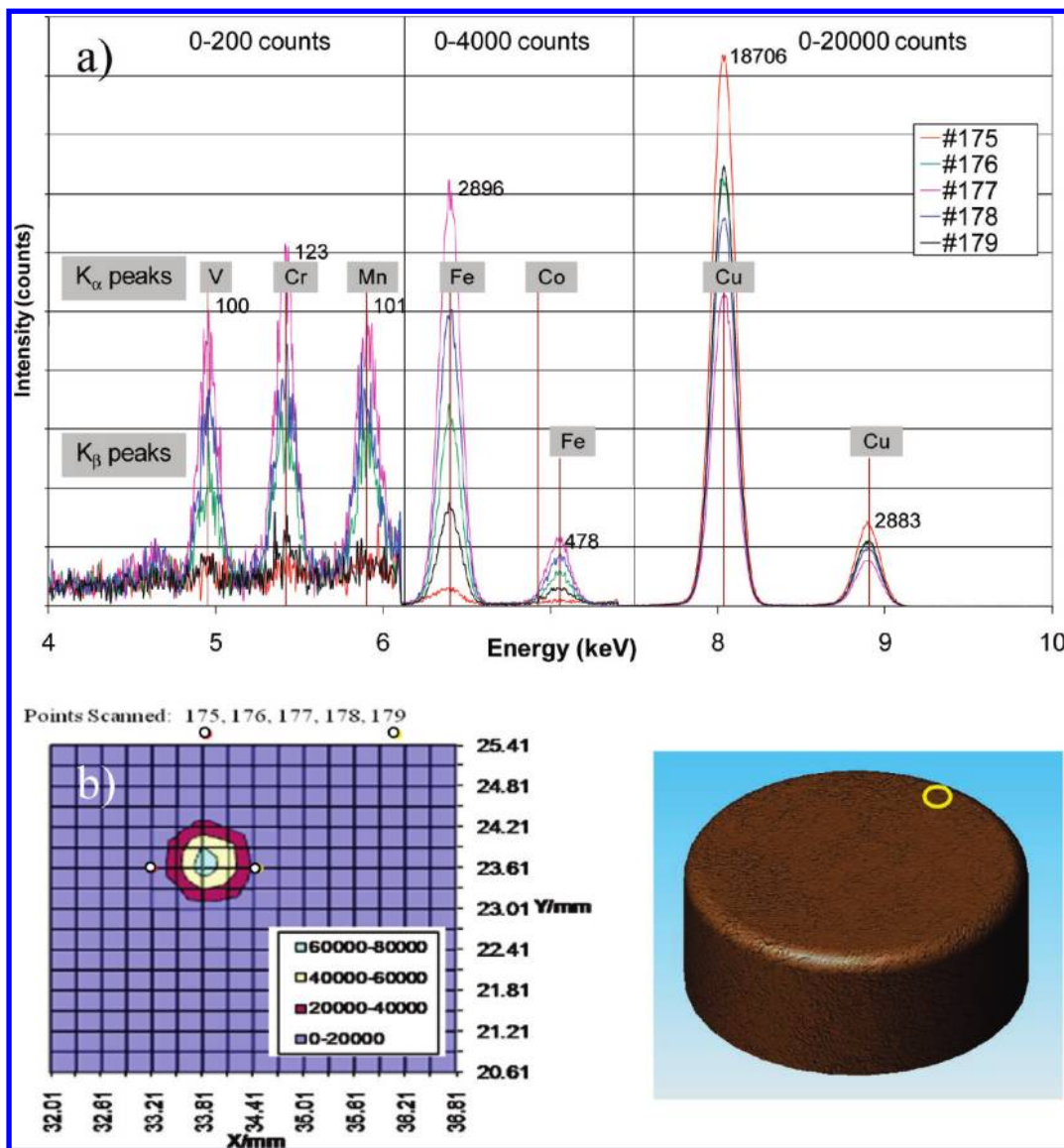
Figure 11. (a) XRF spectra for ingot C for a magnetically active spot located (upper right, yellow circle) near the edge of the bottom of the ingot. (b) Grid pattern in format like Figure 8; white dots mark start (no. 175) and end (no. 179) of grid positions for the five spectra scans (color-coded). For each element, the ordinate scale has been normalized to the intensity observed at no. 177, in order to exhibit most clearly that the Cu K_{\alpha} and K_{\beta} intensities vary the same way but opposite to the SE intensities. Raw pulse counts are shown for grid position no. 177. ARTAX parameters are the same as in Figure 8.
