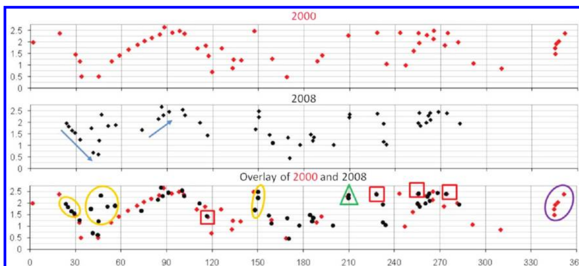
Figure 6. Spots of magnetic attraction are displayed for tailored copper ingot 14-00-01 (see Figure 5) for the years 2000 and 2008. Bottom panel shows an overlay. Red dots denote 2000 data, black dots denote 2008 data. Some spots (enclosed in red boxes) appear identical (i.e., moved less than 1 mm). Some clustered spots seen in 2000 (purple oval) had disappeared by 2008, while three new clusters appeared (orange ovals). One spot (in green triangle) appeared to split into two. The grid height is 2.625 in., and the grid length is 23.25 in.
